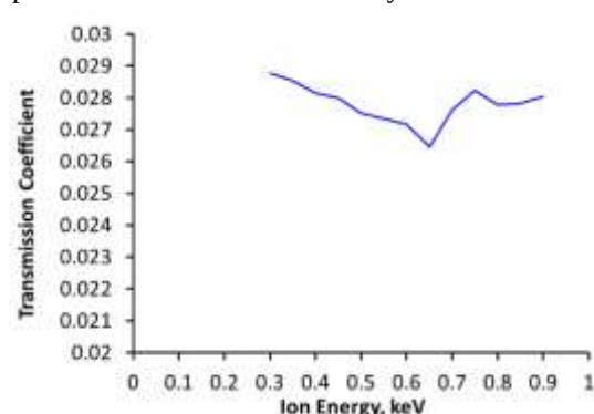
Figure 12. Example transmission coefficient as function of beam voltage for an aligned-grid RPA.
