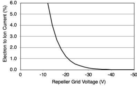
Figure 3. Percentage of electron to ion current flow thru the electron repelling grid as a function of repelling grid voltage showing the onset of electron leakage to the collector region as the repelling voltage is decreased).
