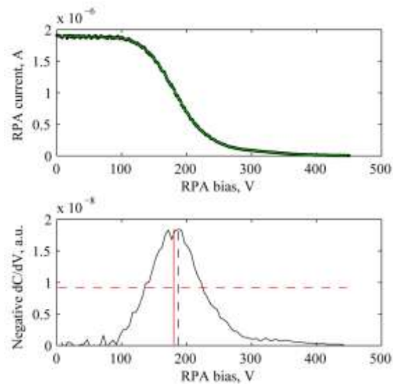
Figure 11. Example of RPA data analysis from an HET operating at 200 V, 10 kW [12]. Top: collector current plotted as a function of discriminator grid bias. Bottom: negative derivative of the collector current as a function of discriminator grid bias.
